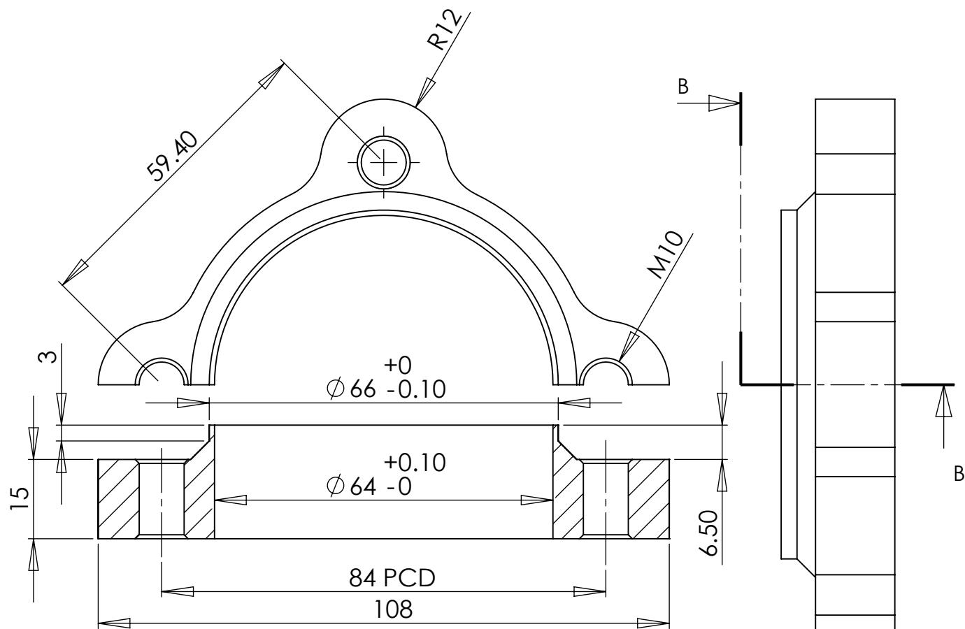
SECTION B-B
